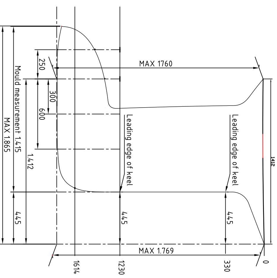
Principle of vertical maximum templates for the X-35 keel
